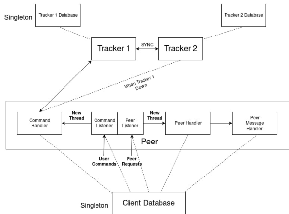
Figure 1: P2P Sharing Data
